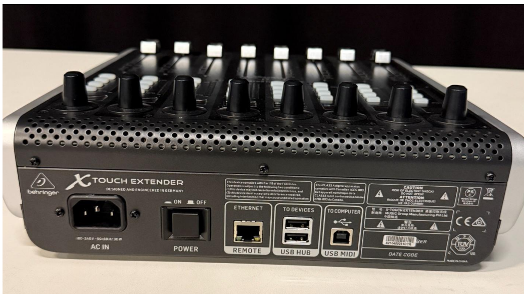
X-Touch Extender - rear connection panel
