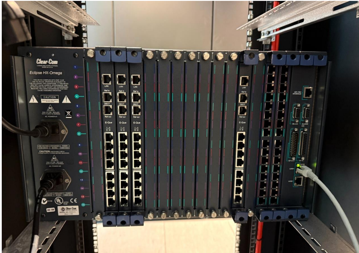
Rear card interfaces / E-Que section
