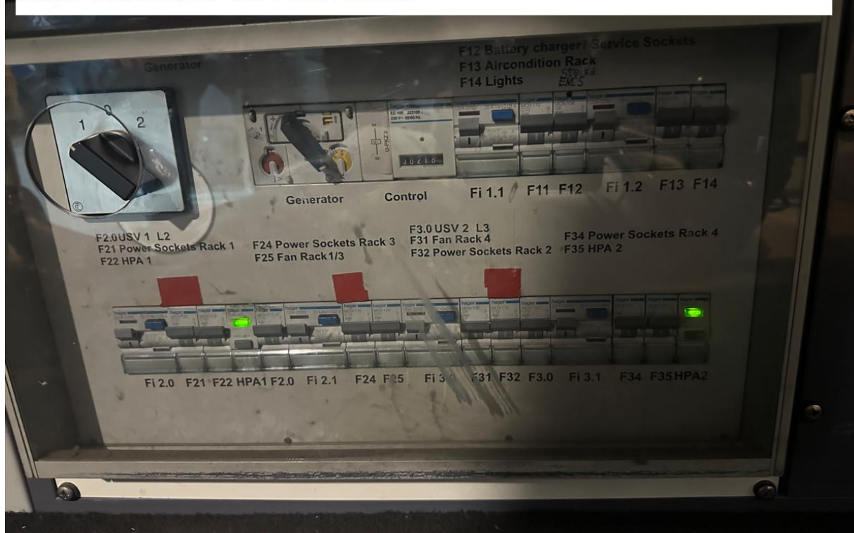
16Ampere CEE power system - not IEC 60364-7-717 ready
