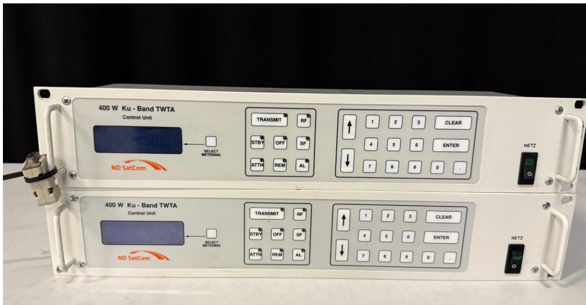
ND SatCom 400 W Ku-Band TWTA control units - front view
